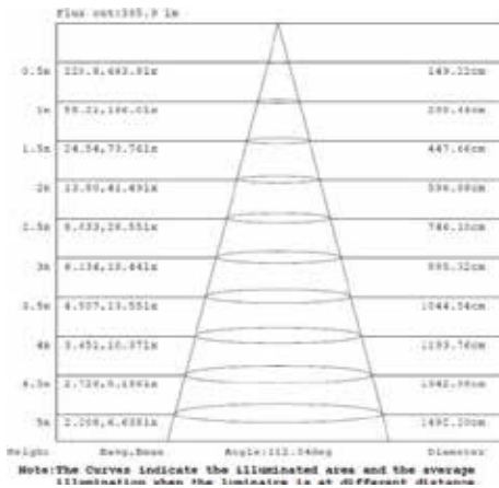
Photometric curve
