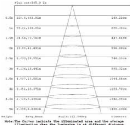
Photometric curve
