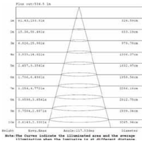
Photometric curve
