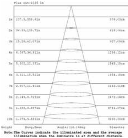
Photometric curve
