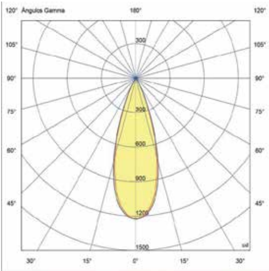
Photometric curve
