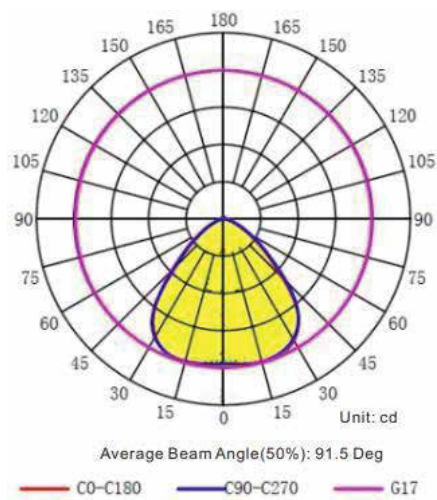
Photometric curve
