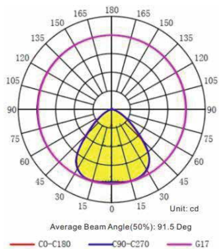
Photometric curve
