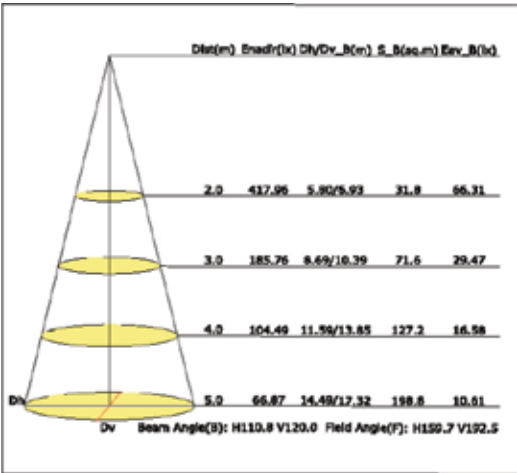
Photometric curve
