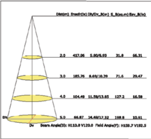
Photometric curve
