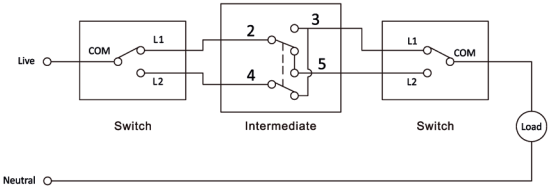
Pattern No.:7 SBL : 200W WIRING DIAGRAMS
