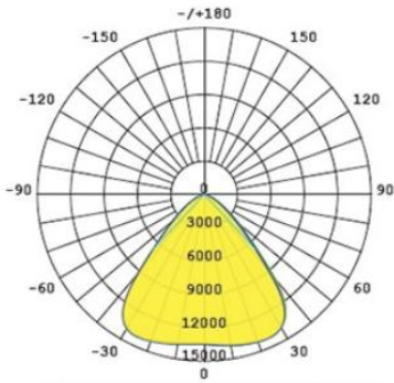
Photometric curve
