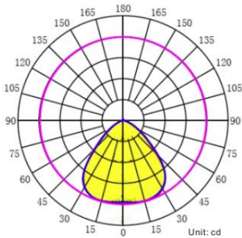
Photometric curve
